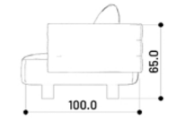
Two seater - Side view - 2S
